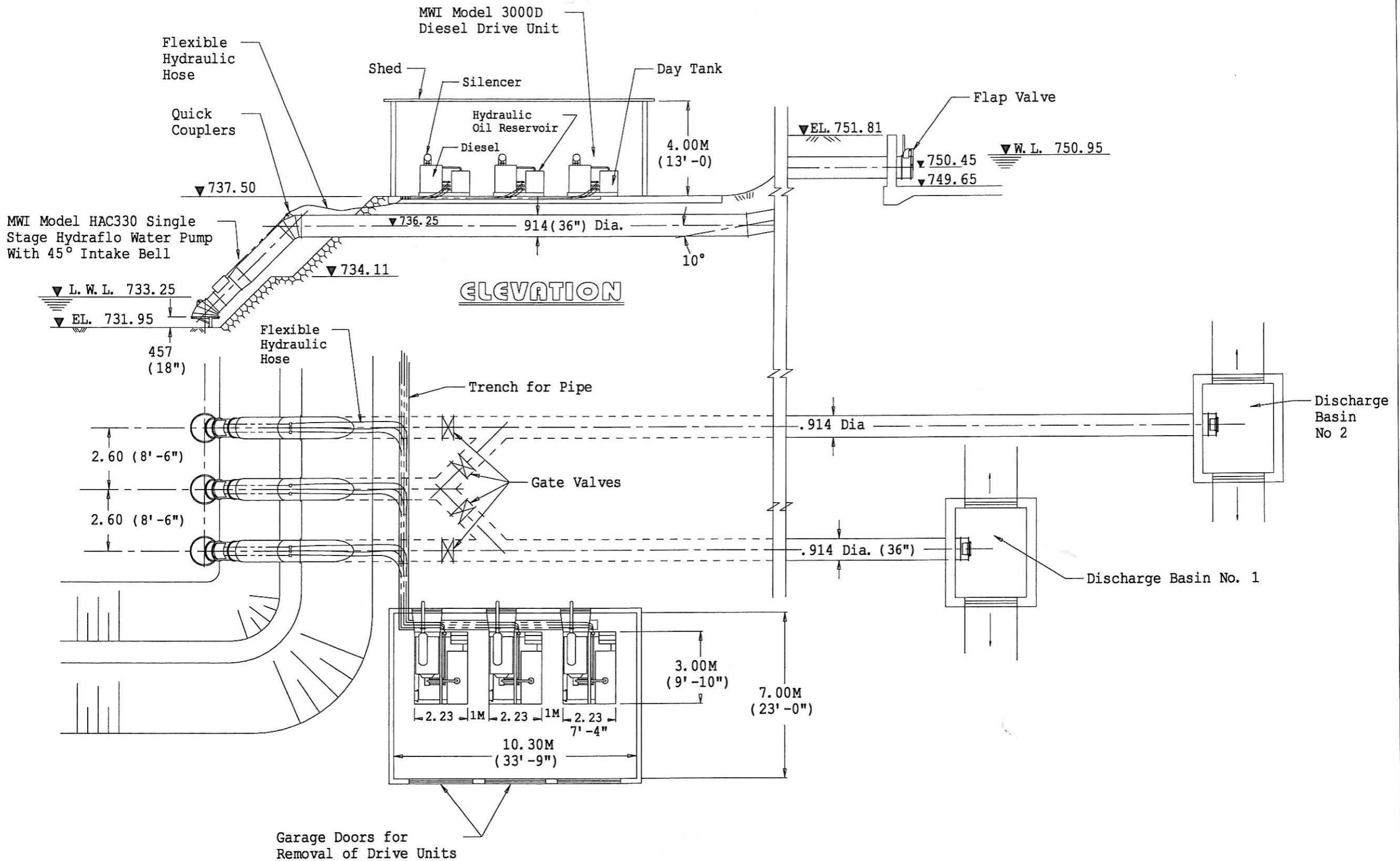
PLAN VIEW
