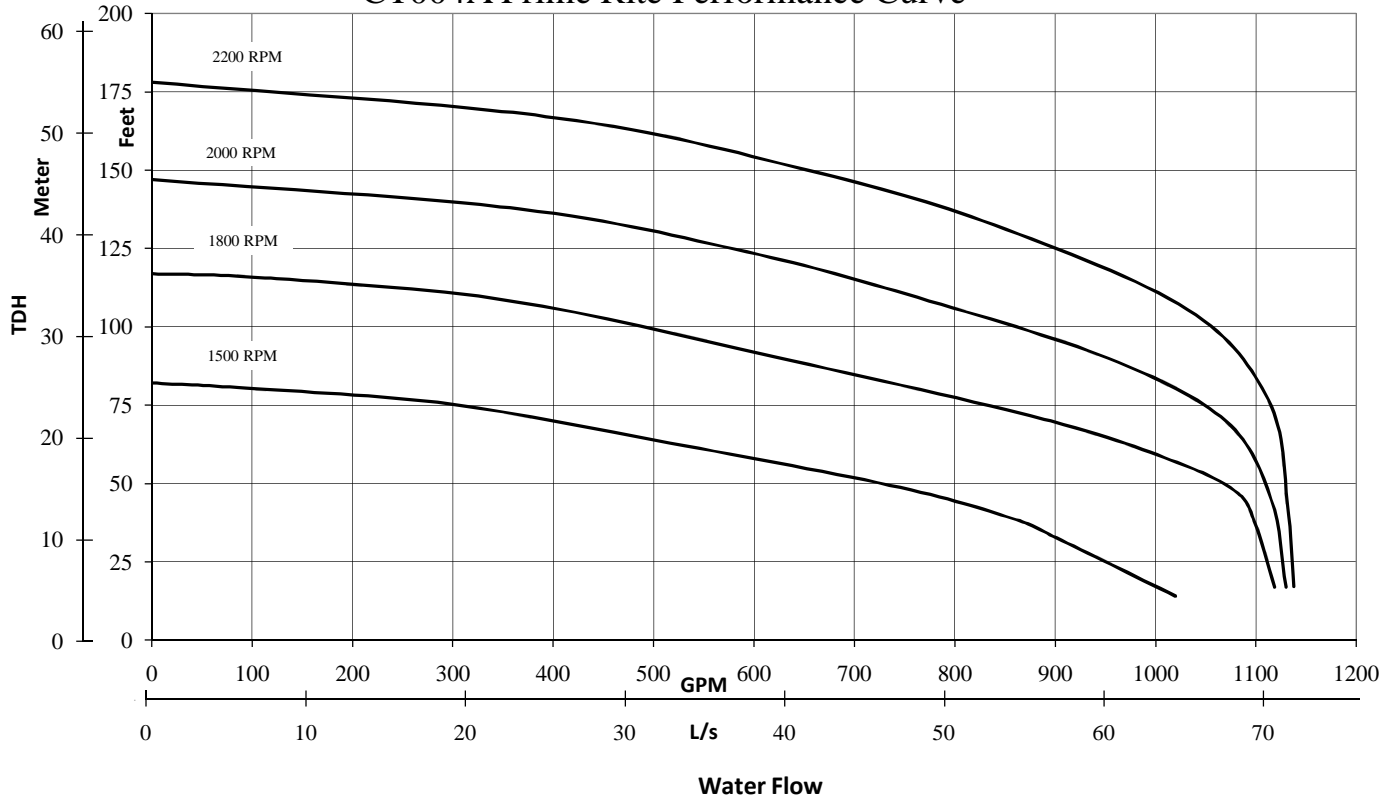
CT004A Prime Rite Performance Curve
